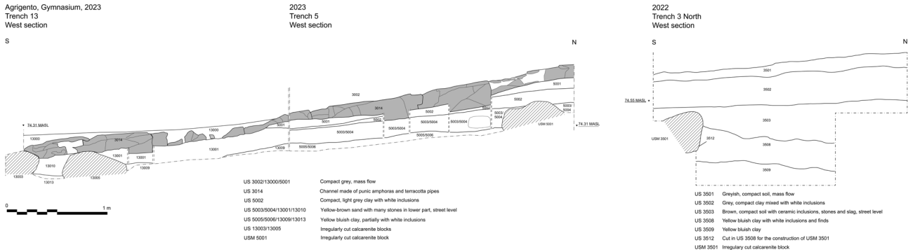
Fig. 4. Stenopos west sections: trench 3N, trench 5, trench 13 (B. Kupke, M. Trümper, J. Winzek).
