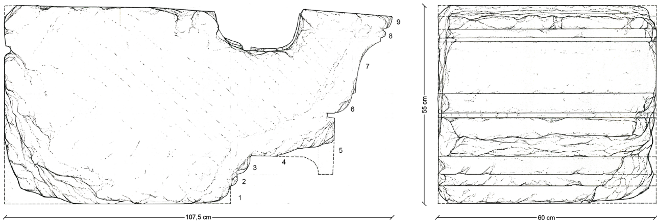
Fig. 46. Cornice with sima, C16: 1. fillet/fascia; 2. half-round; 3. half-round; 4. geison ; 5. geison fascia ; 6. hawkbeak ; 7. sima/cavetto ; 8. half-round; 9. ovolo (M. Delfino).
